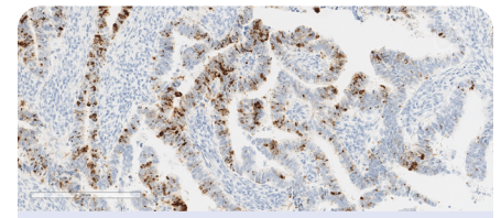
CISH/ISH: HPV16
